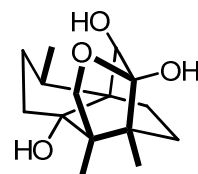
11-O-debenzoyl tashironin
