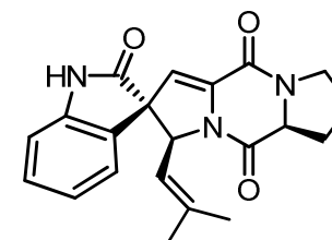
spirotryprostatin B
