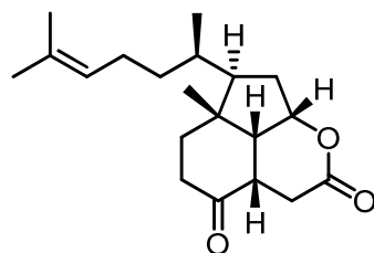
aplykurodinone-1
