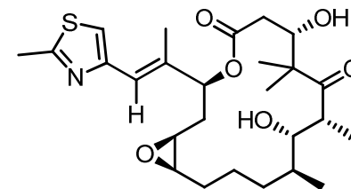
epothilon A
