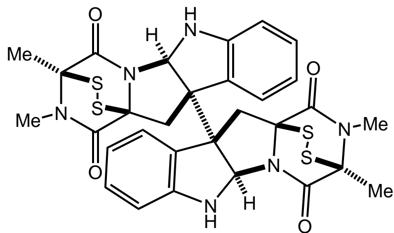
(+)-11,11'-dideoxyverticillin A
